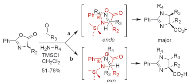
Scheme 1. Proposed Transition States for Diastereoselective Synthesis of anti -Imidazolines
