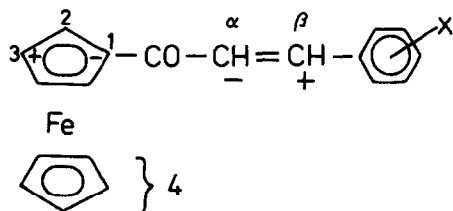
3-aryl-1-ferrocenyl-2-propene-1-one ( X = H )
