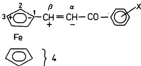
1-aryl-3-ferrocenyl-2-propene-1-one ( X = H )
