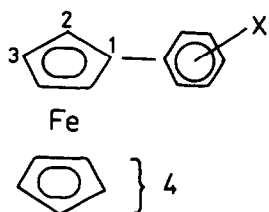
Phenylferrocene ( X = H )
