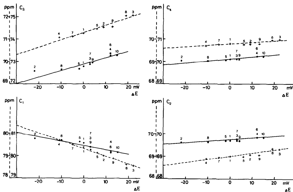
Fig. 4. Chemical shifts of C(1), C(2), C(3) and C(4) of Series II and III as a function of \Delta E . (Dashed curve for Series II.) The substituents are indicated by arabic numbers (Tables 2 and 3).
