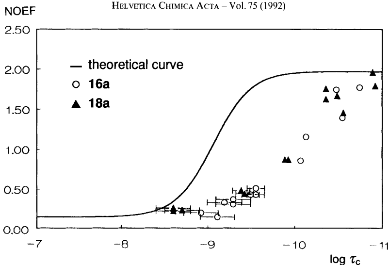
Fig. 6. Plot of the experimental points and the theoretical curve giving the NOEFs as a function of the correlation time \tau_c for B_{CD}^O COOEt ( 16a ) and B_{CD}^O COOEt ( 18a ). The experimental points and theoretical curve were obtained as indicated in Table 6.
