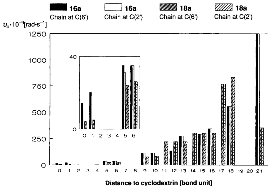
Fig. 5. Plot of the reorientation rate \nu_c (inverse of the correlation time \tau_c ) as a function of the distance from the \beta -cyclodextrin core. The distance is expressed in bond units as defined in Formula 16a and 18a.
