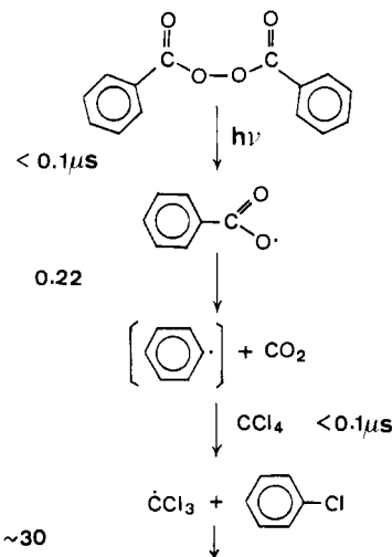
Figure 8. Determined reaction mechanisms for dibenzoyl peroxide in \text{CCl}_4 .
