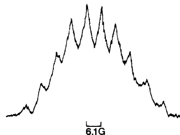
Figure 3. Time-resolved EPR spectrum of 4-iodomethoxybenzene in \text{CCl}_4 at room temperature at 0.4 \mu\text{s} after laser excitation.
