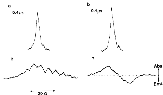
Figure 4. Time-resolved EPR spectra for aerated systems for (a) di-benzoyl peroxide and (b) bis(4-methoxybenzoyl) peroxide in \text{CCl}_4 at room temperature.
