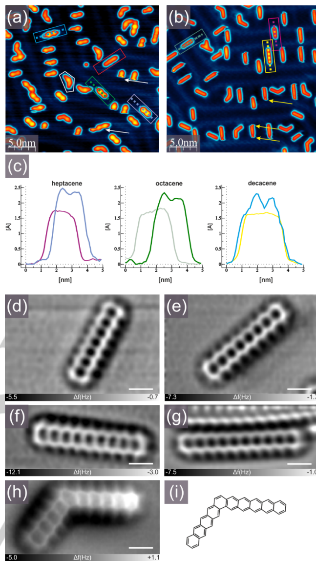
Figure 1. On-surface generation of higher acenes; (a-b) empty state STM images of the Au(111) surface partially covered with (a) hydrogen protected acene precursors 1a , 1b , and 1d , and kinked isomer 1d' , and (b) heptacene ( 2 ), octacene ( 3 ), decacene ( 5 ) and kinked decacene isomer ( 5' ). Precursor molecules are easily discernible by the presence of two pronounced lobes corresponding to two non-aromatic rings each containing two methylene groups, exemplary precursors are marked by rectangles: 1a – violet, 1b – green, 1d – blue. Parent acenes in (b) are indicated by rectangles: 2 – purple, 3 – grey, 5 – yellow. Dashed lines in (a) and (b) indicate directions of profile lines shown in (c); after deposition a small fraction of molecules could be found already partially (white contour) or very rarely completely dehydrogenated (red rectangle). White and yellow arrows in (a) and (b) indicate the typical displacement of precursors and frustrated motion of acenes during STM imaging, respectively. Tunneling current 30 pA, bias voltage + 2.0 V; (c) profile lines along precursor molecules and parent acenes clearly showing a difference in their STM appearance and evidencing the presence of two pronounced lobes in the topographies of the precursors; (d-h) Laplace filtered constant height, frequency shift nc-AFM images of 2 (d), 3 (e), 4 (f), 5 (g), and 5' (h) generated by annealing, scale bar: 5 Å; (i) structural scheme of 5' .
