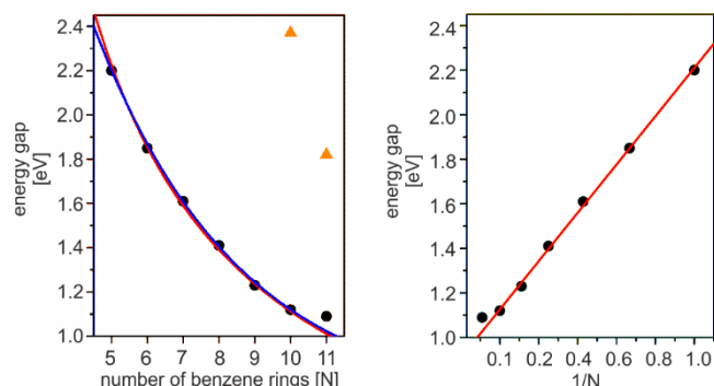
Figure 3. STS measured transport gap for long acenes on Au(111); (a) dependence of the gap on the number of fused benzene rings with the inverse proportionality fit (red curve) and exponential decay (blue curve) for pentacene-decacene data. Values recorded for kinked isomers are displayed by orange triangles [28] ; (b) transport gap drawn as a function of the inversed number of rings with the linear fit for pentacene-decacene data; gap values for pentacene [29] and hexacene [23] are taken from the literature.
