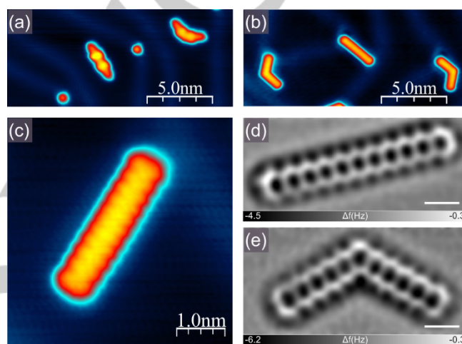
Figure 2. On-surface generation of undecacene ( 6 ); empty state STM images of the Au(111) surface (a) with the mixture of undecacene precursors 1e and 1e' and (b) subsequently thermally generated parent 6 and kinked undecacene isomer 6' . Tunneling current: (a,b) 30 pA, (c) 150 pA, bias voltage + 2.0 V; (c) high resolution filled state STM image of 6 with clearly visible eleven lobes along the molecule, tunneling current 30 pA, bias voltage -1.0 V; (d-e) present Laplace filtered constant height, frequency shift nc-AFM images of 6 (d) and 6' (e); scale bar: 5 Å.
