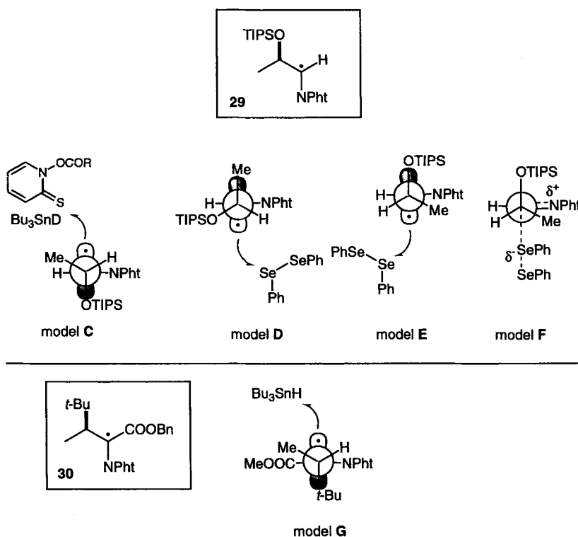
Fig. 2. Models for the stereochemistry of the radical reactions. TIPS = (i-Pr) 3 Si, Ph = phthaloyl.
