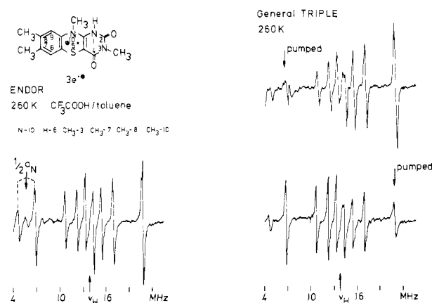
Figure 4. ENDOR (left) and general TRIPLE spectra of the thiaisoalloxazine cation radical 3e^+ : B_{\text{NMR}}(\text{scan}) = 0.4 \text{ mT} (14 MHz); B_{\text{NMR}}(\text{pump}) = 0.4 \text{ mT} .
