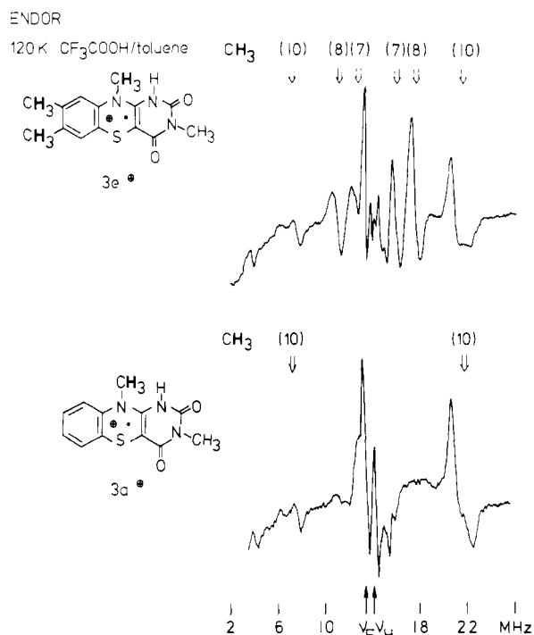
Figure 7. ENDOR spectra in disordered solids of a thiaisoalloxazine and a 7,8-dimethylthiaisoalloxazine cation radical.
