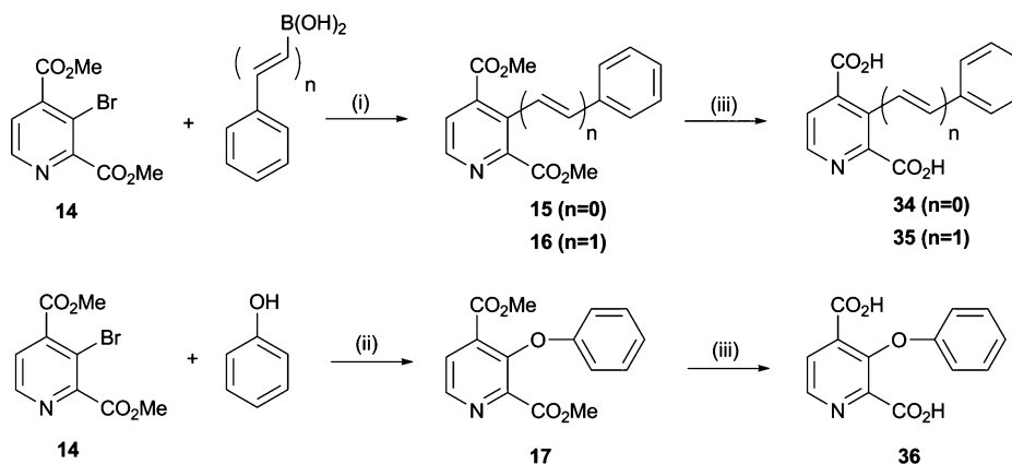
Scheme 3 Synthesis of pyridine dicarboxylate derivatives 34–36 . Reagents and conditions: (i) \text{Pd}(\text{OAc})_2 (10 mol%), \text{PPh}_3 (0.2 eq.), \text{Cs}_2\text{CO}_3 (1.1 eq.), DMF, 70 °C, 3–5 h, 60–75%; (ii) \text{CuI} (0.1 eq.), N -( n -butyl)imidazole (0.5 eq.), \text{Cs}_2\text{CO}_3 (2 eq.), toluene, MW, 140 °C, 1 h, 44%; (iii) \text{NaOH} , \text{MeOH} , \text{H}_2\text{O} , 6 h–overnight, 49–75%.
