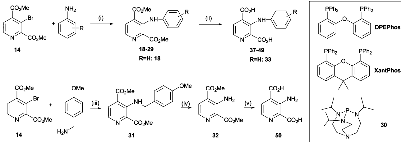
Scheme 4 Synthesis of pyridine dicarboxylate derivatives 37–50 . Reagents and conditions: (i) \text{Pd}(\text{dba})_3 (2 mol%), ligand L (6 mol%), base (1.4 eq.), toluene, MW, 110–150 °C; L = \text{PPh}_3 or BINAP or 30 : <5% conversion; L = DPEPhos: 11% yield; L = XantPhos: 77% yield; (ii) \text{NaOH} , \text{MeOH} – \text{H}_2\text{O} , RT; (iii) \text{Pd}(\text{dba})_3 (2 mol%), XantPhos (6 mol%), \text{Cs}_2\text{CO}_3 (1.4 eq.), toluene, MW, 110 °C, 12 h, 69%; (iv) \text{CF}_3\text{CO}_2\text{H} , \text{CH}_2\text{Cl}_2 , 0 °C to RT, 89%; (v) \text{NaOH} , \text{MeOH} – \text{H}_2\text{O} , 2 h, RT, 67%.
