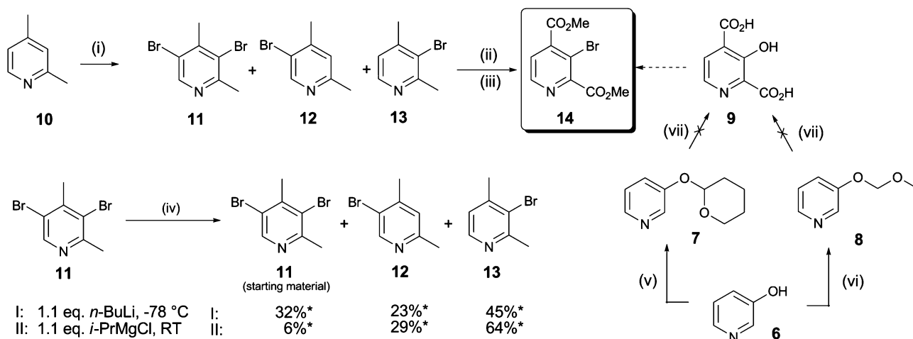
Scheme 2 Synthesis of 3-bromopyridine 14 . Reagents and conditions: (i) \text{Br}_2 (0.9 eq.), 20% oleum, 165 °C, 24 h, 11 (12%), 12 (22%), 13 (35%); (ii) \text{KMnO}_4 (5 eq.), \text{NaOH} (0.7 eq.), \text{H}_2\text{O} , 110 °C, 3 h; (iii) cat. \text{H}_2\text{SO}_4 , MeOH, reflux, 24 h, 53%; (iv) n\text{-BuLi} (1.1 eq.), THF, -78 °C, 1 h, or i\text{-PrMgCl} (1.1 eq.), THF, RT; then MeOH workup; (v) tetrahydropyran-2-ol (1.1 eq.), \text{PPh}_3 (1.1 eq.), diisopropyl azodicarboxylate (1.1 eq.), RT, 2 h, 46%; 23 (vi) methoxymethyl chloride (1.05 eq.), \text{KO}^t\text{Bu} (1.1 eq.), DMF- \text{CH}_3\text{CN} , RT, 1 h; 26 (vii) base (1.5 eq.), then excess \text{CO}_2(\text{s}) ; base (1.5 eq.), then excess \text{CO}_2(\text{s}) ; then HCl/dioxane; *Ratios as determined by ^1\text{H} NMR.
