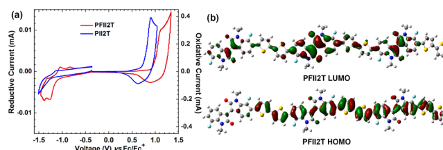
Figure 2. (a) Cyclic voltammograms of both polymers in thin film drop-casted on a glassy carbon electrode. (b) Calculated molecular orbitals of the trimmer of PFII2T (B3LYP/6-31G(d)).
