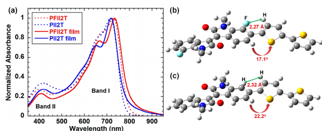
Figure 1. (a) Normalized UV-vis absorption spectra of both polymers in \text{CHCl}_3 ( 1 \times 10^{-5} M) and in thin film. Molecular models of (b) PFII2T and (c) PII2T fragments. Alkyl chains were replaced by methyl groups for simplicity (geometries were optimized at B3LYP/6-31G(d) level). PFII2T displays smaller dihedral angle ( 17.1^\circ ) and shorter F–H distance (2.27 Å).
