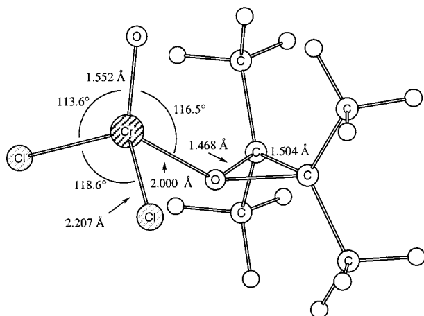
Figure 3. Optimized C_s ( 3A' ) structure calculated for \text{OCrCl}_2 \cdots \text{TMEO} , 7 , by means of DFT calculations using SV(P) basis sets (B3LYP). Selected bond lengths and angles are given in angstroms and degrees, respectively.
