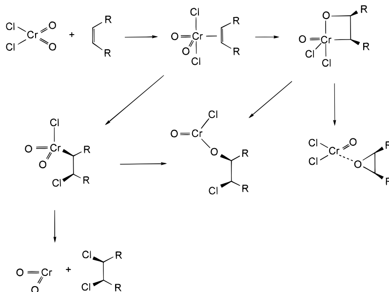
Scheme 1. Postulated Mechanism for the Thermal Olefin Oxidation with \text{CrO}_2\text{Cl}_2 13
