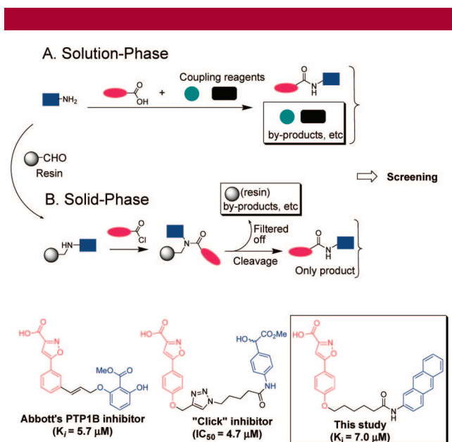
Figure 1. (a) Two strategies using amide bond-forming reaction. (b) Various cell-permeable PTP1B inhibitors. The bidentate inhibitors contain a core (in red) and a peripheral group (in blue).
