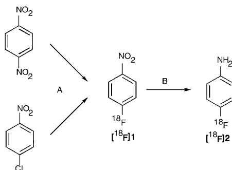
Scheme 2. Preparation of para- ^{18}\text{F} fluoroaniline; (A) [\text{K}/2.2.2][^{18}\text{F}]\text{F} , \text{K}_2\text{CO}_3 , DMSO, 120^\circ\text{C} , 3 min; (B) Pd black, \text{H}_3\text{PO}_3 , MeOH, reflux, 15 min
