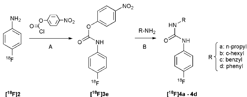
Scheme 4. Preparation of 4-[ 18 F]fluorophenylcarbamate nitrophenyle ester and N-4-[ 18 F]fluorophenyl-N'-substituted ureas; (A) THF, Na 2 SO 4 -cartridge, (B) THF, Δ
