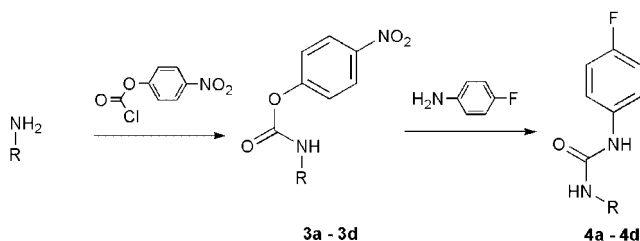
Scheme 6. Preparation of carbamate 4-nitrophenylesters and 4-fluorophenyl ureas; a–d, see Scheme 4
