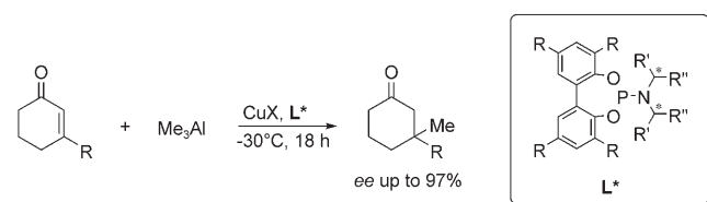
Scheme 1. Copper-catalyzed A.C.A. of \text{Me}_3\text{Al} to 3-substituted cyclohex-2-enones.
