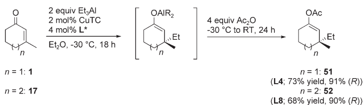
Scheme 7. Tandem Cu-catalyzed A.C.A. of Et_3Al - O -acylation.
