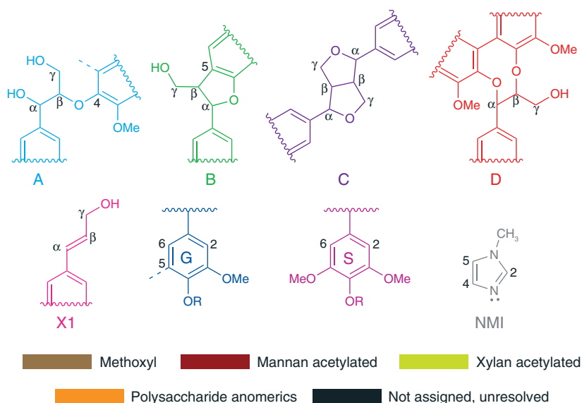
Figure 3. Key to the chemical structures found in the spectra in Figs 4–7. The structures are: (A) \beta -aryl ether in cyan, (B) phenylcoumaran in green, (C) resinol in purple, (D) dibenzodioxocin in red, (X1) cinnamyl alcohol endgroups in magenta, (G) guaiacyl in dark blue, (S) syringyl in fuchsia, and (NMI) 1-methylimidazole in gray. Other structures include: lignin methoxyl in brown, H-2/C-2 & H-3/C-3 correlations for the acetylated structure of \beta -D-Manp l in maroon, H-2/C-2 & H-3/C-3 correlations for the acetylated structure of \beta -D-Xylp l in chartreuse, polysaccharide anomers in orange, and structures currently not assigned or unresolved in black.
