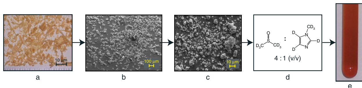
Figure 1. A diagram illustrating the nonderivatized dissolution of plant cell walls. Pinus taeda is shown here as an example: a, shavings produced via conventional planer; b, cryogenically mixer-milled; c, planetary ball-milled; d, dissolution method; e, NMR tube of cell walls in solution.
