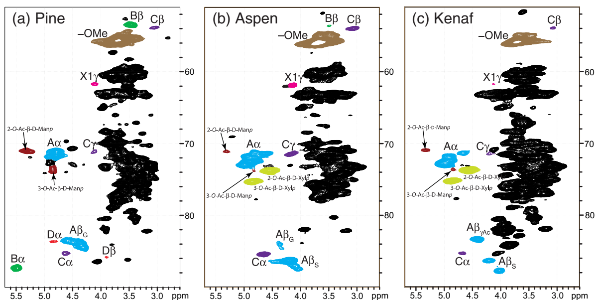
Figure 5. Aliphatic region of the whole plant cell wall HSQC spectra: a, pine; b, aspen; and c, kenaf. The black contours are currently unresolved, mostly because of heavy overlapping in these regions. All contour colors and labels can be matched to their respective structure in Fig. 3. As noted in the text, A\beta_G is any syringyl or guaiacyl coupled to a guaiacyl \beta -aryl ether, A\beta_S is any syringyl or guaiacyl coupled to a syringyl \beta -aryl ether, and A\beta_{\gamma Ac} is a tentative assignment for a \beta -aryl ether linkage with a \gamma -acetate. 2-O-Ac- \beta -D-Manp, H-2/C-2 correlation for the acetylated structure of \beta -D-Manp [32] ; 3-O-Ac- \beta -D-Manp, H-3/C-3 correlation for the acetylated structure of \beta -D-Manp [32] ; 2-O-Ac- \beta -D-Xylp, H-2/C-2 correlation for the acetylated structure of \beta -D-Xylp [30,31] ; 3-O-Ac- \beta -D-Xylp, H-3/C-3 correlation for the acetylated structure of \beta -D-Xylp [30,31] .
