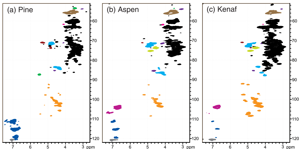
Figure 4. HSQC spectra from nonderivatized plant cell walls: a, pine; b, aspen; and c, kenaf at 500 MHz. Note that the spectra cover the range for all the cell wall components – cellulose, hemicelluloses, and lignin. All contour colors can be matched to their respective structures in Fig. 3. Expanded regions are shown in Figs 5–7.
