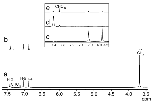
Figure 2. Proton spectra of various stages in NMI deuteration: a, 1-methylimidazole; b, 1-methyl- d_3 -imidazole; c, ring deuteration as per Hardacre et al. [27] ; d, ring deuteration as per Esaki et al. [28] ; e, ring deuteration with combination of methods.
