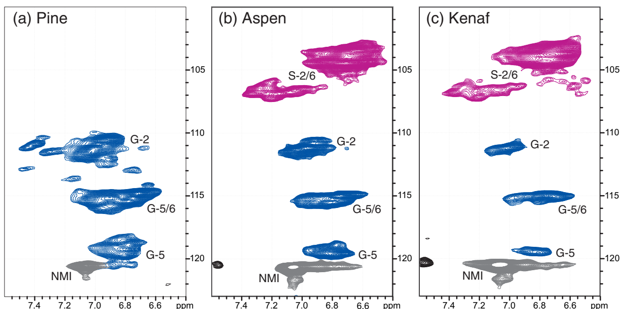
Figure 6. Aromatic region of the whole plant cell wall HSQC spectra: a, pine; b, aspen; and c, kenaf. The guaiacyl and syringyl contours are a combination of free phenolic and etherified aromatic units. Contour colors and labels can be matched to their respective structure in Fig. 3.
