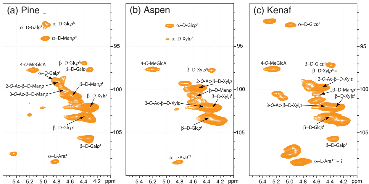
Figure 7. Anomeric region of the whole plant cell wall HSQC spectra: a, pine; b, aspen; and c, kenaf. Assignments are as follows: \beta -D-GlcP I , internal \beta -D-glucopyranoside units (cellulose) [31–33] ; \beta -D-ManP I , internal \beta -D-mannopyranoside units [32,33] ; \beta -D-XylP I , internal \beta -D-xylopyranoside units [30] ; \alpha -D-Galp T , terminal \alpha -D-galactopyranoside units [32,33] ; \beta -D-Galp T , terminal \beta -D-galactopyranoside units [33] ; \alpha -L-Araf T , terminal \alpha -L-arabinofuranoside units [31,32,50] ; 2-O-Ac- \beta -D-ManP, anomeric correlation for the acetylated H-2/C-2 structure of \beta -D-ManP I ; 3-O-Ac- \beta -D-ManP, anomeric correlation for the acetylated H-3/C-3 structure of \beta -D-ManP I [32] ; 2-O-Ac- \beta -D-XylP, anomeric correlation for the acetylated H-2/C-2 structure of \beta -D-XylP I [30,31] ; 3-O-Ac- \beta -D-XylP, anomeric correlation for the acetylated H-3/C-3 structure of \beta -D-XylP I [30,31] ; 4-O-MeGlcA, 4-O-methyl- \alpha -D-glucuronic acid [30] ; \alpha and \beta -D-GlcP R , reducing ends of glucopyranoside [32,33] ; \beta -D-ManP R , reducing end of mannopyranoside [32] ; \alpha and \beta -D-Galp R , reducing ends of galactopyranoside [33] ; \alpha and \beta -D-XylP R , reducing ends of xylopyranoside [30] .
