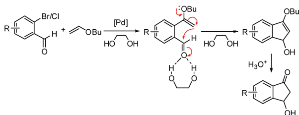
Scheme 1. Working Hypothesis for Accessing 1-Indanones
