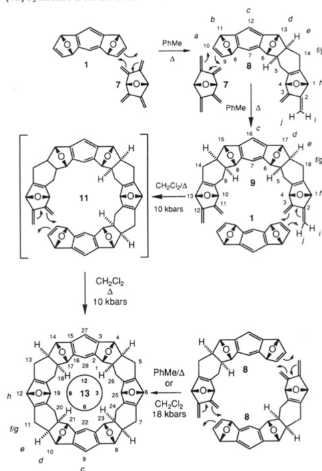
Scheme III. Molecular LEGO Set Used for the Synthesis of the [12]Cyclacene Derivative 13 a
