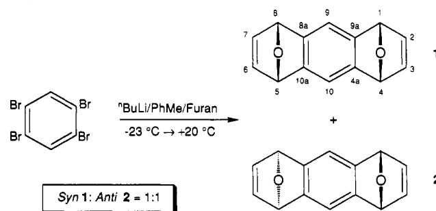
Scheme 1. Synthesis of the syn - and anti -Bisdienophiles, 1 and 2 , Respectively a
