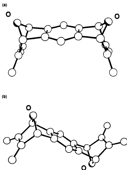
Figure 10. X-ray crystal structures of (a) the syn and (b) the anti extended bisdienes, 26 and 27 , respectively. The concave/convex nature of the syn -bisdienophile 26 is clearly visible.
