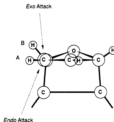
Figure 3. A Newman projection along a selected carbon (olefinic)—carbon (bridgehead) bond in a structural fragment of the syn -bisdienophile 1. This shows the torsional interaction associated with the olefinic (A) and the adjacent bridgehead (B) hydrogen atoms. More important in the context of the treble diastereoselective Diels–Alder reaction is the staggering of the bonds under construction at the exo face and the vicinal bonds located on the bridgehead carbon atoms.
