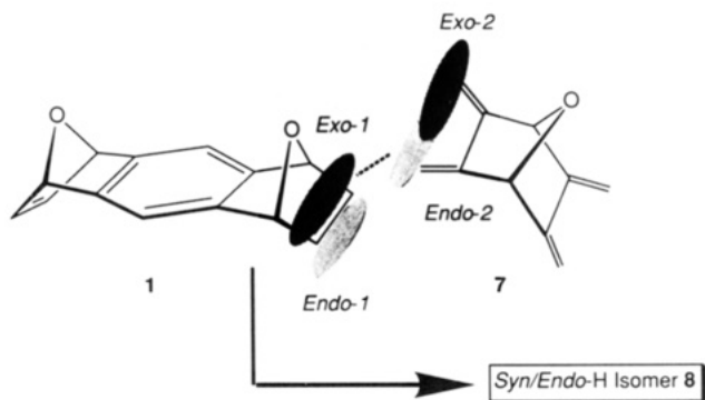
Figure 5. By uniting the factors which govern the reactivities and selectivities of the building blocks 1 and 7 , a qualitative understanding of the origin of the diastereoselectivities exhibited in their mutual reaction can be acquired. Combining \pi -faces of high (dark) and low (light) electron densities in a manner that allows reaction at the exo face (exo-1) of the bisdienophile 1 and at the endo face (endo-2) of the bisdiene 7 generates the observed 1:1 adduct 8 , with syn/endo-H stereochemistry across the newly-formed cyclohexene ring via a syn/exo-1/endo-2 transition state. The only other mode by which this stereochemistry could be attained would be by reaction between exo faces on both the bisdienophile 1 and the bisdiene 7 , i.e., via a syn/exo-1/exo-2 transition state. Apart from bringing two \pi -faces of high electron density together, this transition state would have to encounter very serious steric interactions between the two endoxide bridges in the two reactants. Steric interactions presumably disfavor the only other transition state—viz. the anti/exo-1/endo-2 one—that would allow reaction to take place between the exo face (exo-1) of the bisdienophile 1 and the endo face (endo-2) of the bisdiene 7 . Note that the “1” and “2” following exo and endo refer to “ene” and “diene”, respectively.
