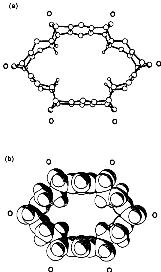
Figure 7. The X-ray crystal structure of the [12]cyclacene derivative that we have dubbed kohnkene 13. The closed macropolycyclic structure is clearly visible in the (a) ball-and-stick and (b) space-filling representations.
