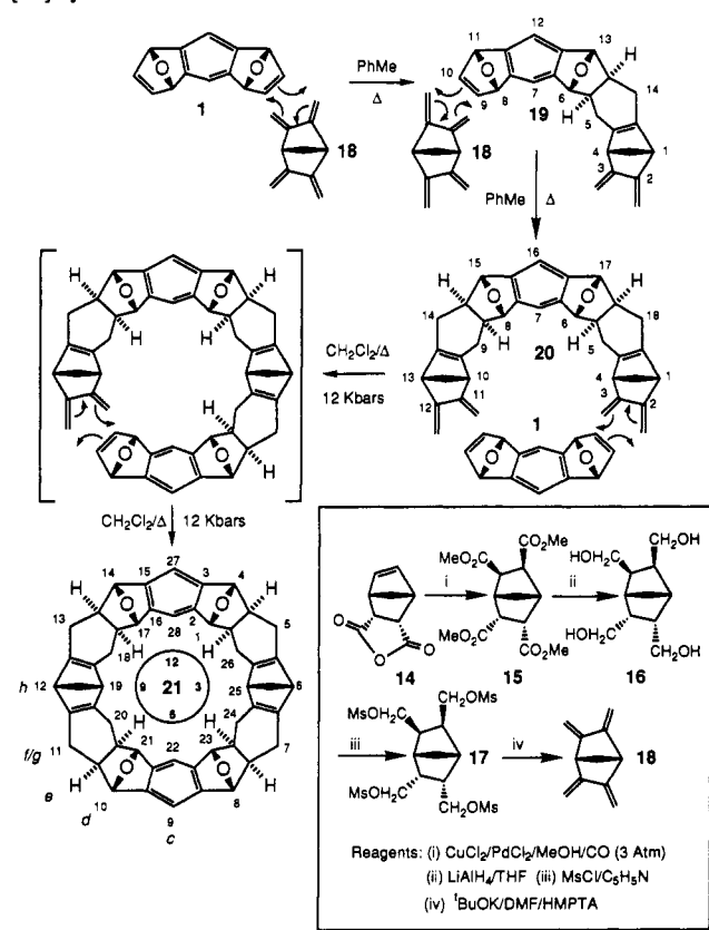
Scheme V. The Molecular LEGO Set Used for the Synthesis of the [12]Cyclacene Derivative 21 a
