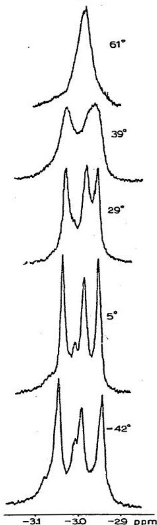
Fig. 2. Proton NMR patterns at various temperatures of a chloroform solution of \text{As}_4(\text{NCH}_3)_6 \cdot \text{Ni}(\text{CO})_3 complexes, with the solution being one molar in total \text{As}_4(\text{NCH}_3)_6 and an \text{Ni}(\text{CO})_3/\text{As}_4\text{N}(\text{CH}_3)_6 mole ratio of ca. 0.83.
