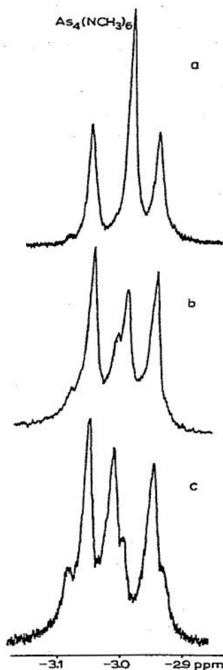
Fig. 3. Proton NMR spectra obtained at -40^\circ on chloroform solutions of \text{As}_4(\text{NCH}_3)_6 \cdot \text{Ni}(\text{CO})_3 where the solution is one molar in total \text{As}_4(\text{NCH}_3)_6 and there are increasing amounts of nickel carbonyl. Spectra a, b, and c correspond respectively to \text{Ni}(\text{CO})_3/\text{As}_4(\text{NCH}_3)_6 mole ratios of ca. 0.69, 0.83, and 1.4, as calculated from the amount of reagents used or from the carbon-monoxide evolution. Values of 0.61, 0.85, and 1.3, respectively, were estimated from the relative peak areas in the NMR spectra.
