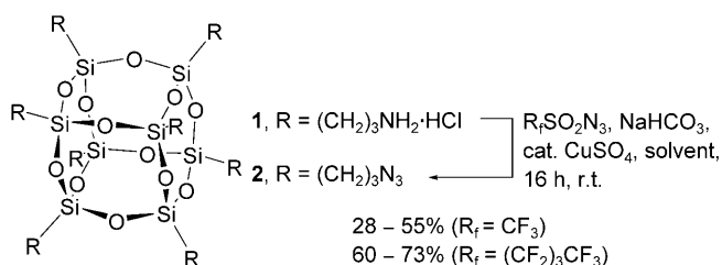
Scheme 1. Synthesis of octa-azide 2 using \text{TfN}_3 and \text{NfN}_3 .
