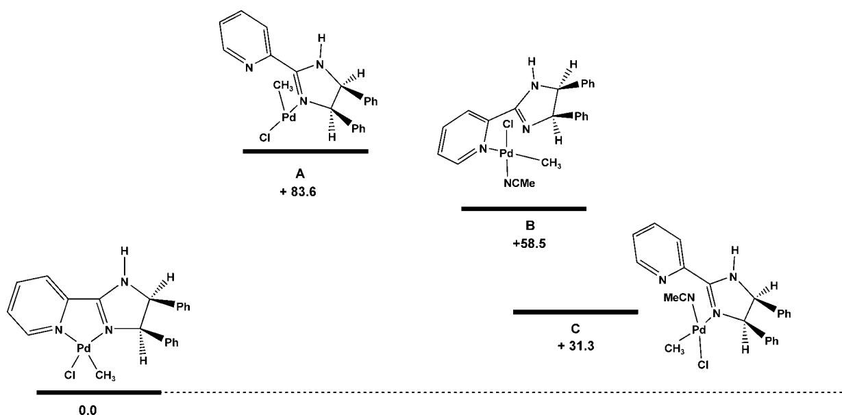
Figure 6. Selected intermediates for the dissociative pathway. [energies in \text{kJ mol}^{-1} ].
