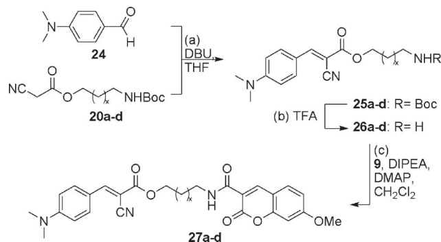
Scheme 3 Reagents and conditions: (a) 1.0 equiv. 24 , 1.1 equiv. 20 , 1.16 equiv. DBU, THF, 18 h, 25 °C, 62–82%; (b) 1.0 equiv. 25 , TFA/ CH_2Cl_2 , 30 min, 25 °C; (c) 1.1 equiv. 26 , 1.0 equiv. 9 , 2.0 equiv. DIPEA, 0.1 equiv. DMAP, CH_2Cl_2 , 18 h, 25 °C, 64–78% (over two steps).
