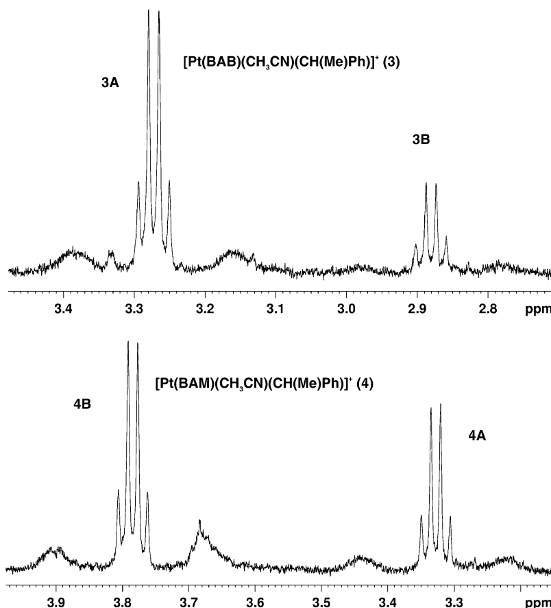
Figure 4. ^1\text{H} NMR spectra in \text{CD}_2\text{Cl}_2 showing the chemical shifts and the relative intensity of the \text{CH}(\text{Me}) proton of the two diastereomers in 3 and 4 in the reaction mixtures.
