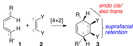
Figure 1. Stereochemistry of Diels–Alder reactions.
