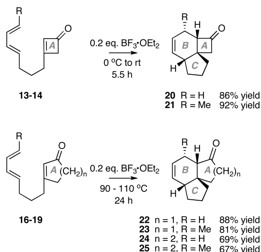
Figure 5. Lewis acid (LA)-catalyzed IMDA reactions.
