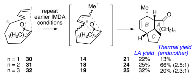
Figure 7. Tandem diene migration-IMDA. Thermal and Lewis acid (LA)-catalyzed IMDA conditions for the appropriate dienophile ring size are as shown in Figures 5 and 6.
