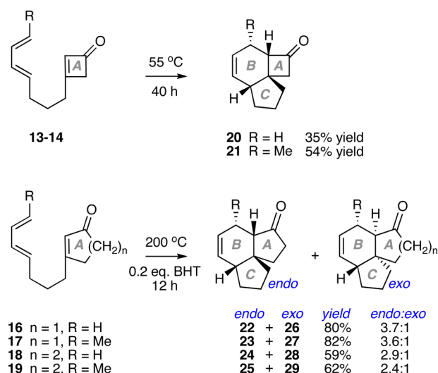
Figure 6. Thermal IMDA reactions.
