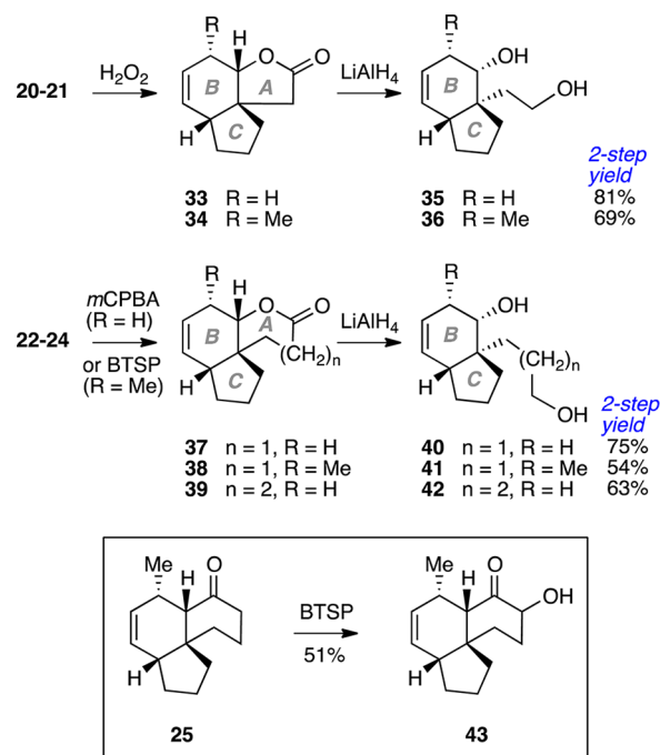
Figure 8. Illustrative fragmentation of A-ring to trans BC hydrindenenes.
