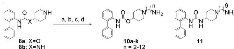
Scheme 2. Reagents and conditions: (a) bromoalcohol, DIPEA, DMF, 50 °C, 49–82%; (b) DMSO, \text{Py}\cdot\text{SO}_3 , DIPEA, DCM, 0 °C, 60–90%; (c) dibenzylamine, \text{Na}(\text{OAc})_3\text{BH} , 1:1 DCM–MeOH, 70–85%; (d) \text{H}_2 , cat Pd(OH) 2 , EtOH, 70–90%.
