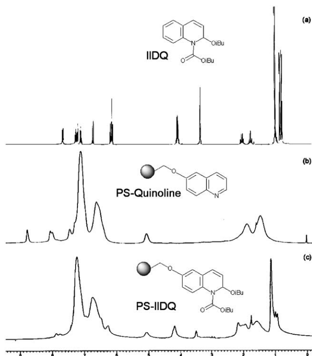
Fig. 1 NMR spectra at 400 MHz showing evidence of the synthesis of PS-IIDQ.
