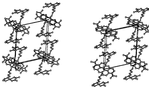
Figure 2. Stereoview of the unit cell of [\text{Pt}\{\text{AO}(\text{CH}_2)_6\text{en}\}(\text{ox})](\text{NO}_3) \cdot 7\text{H}_2\text{O} ( 10 ). The nitrate anions and water molecules are omitted for clarity. View is along the [001] axis.
