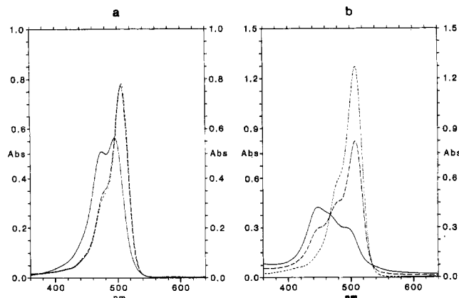
Figure 3. Visible absorption spectra of (a) [Pt{AO(CH 2 ) 6 en}Cl 2 ]Cl ( 9 ) and (b) [Pt{AO(CH 2 ) 3 en}Cl 2 ]Cl ( 20 ) in the absence (—) of DNA, immediately after addition to a DNA solution (---), and after a 48-h incubation (···) of the drug/DNA solution. The buffer in all samples is 10 mM sodium cacodylate, 6.6 mM Tris-HCl, 1.65 mM Na 2 EDTA, pH 7.2. The calf thymus DNA phosphate concentration is 431 \mu M, and the concentration of the intercalator is \sim 13.5 \mu M, giving D/N = 0.031.
