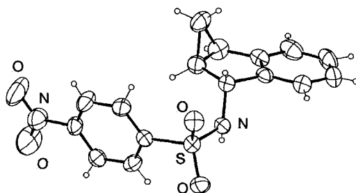
Fig. 1. Perspective view of the crystal structure of 4-nitro-N-[(1aRS,6RS,6aSR)-1,1 \alpha ,6,6 \alpha -tetrahydrocycloprop[a]inden-6-yl]benzenesulfonamide ( 36 ). Ellipsoids are represented at 50% probability level.
