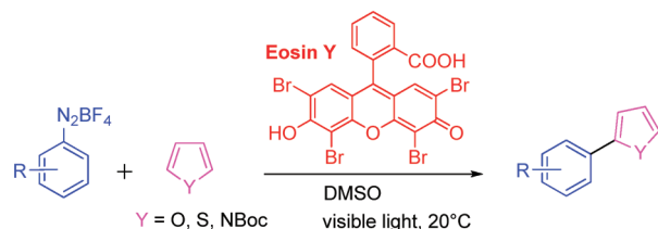
Figure 1. Metal-catalyzed and photocatalytic approaches for direct C–H arylation of heteroarenes.
