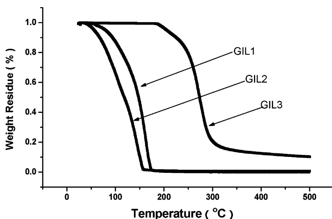
Figure 2. TGA curves of GILs 1–3.
