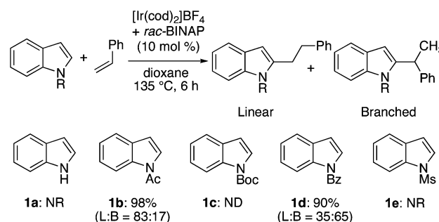
Scheme 1. Relative Reactivity of N -Substituted Indoles
