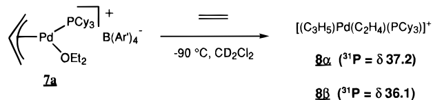
Scheme 2. In Situ Generation of Isomeric [(\text{C}_3\text{H}_5)\text{Pd}(\text{C}_2\text{H}_4)(\text{PCy}_3)]^+[\text{B}(\text{Ar}')_4]^- ( 8a and 8b )
