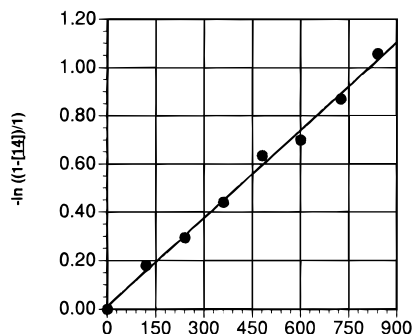
Figure 5. The -\ln[(A_0 - B)/(A_0 - B_0)] versus time data for allyl acrylate coupling of complex 13 .
