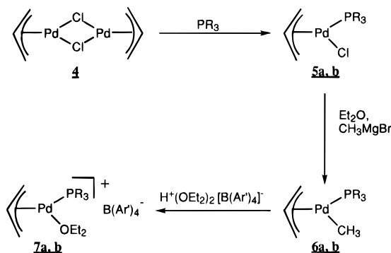
Scheme 2. In Situ Generation of Isomeric [(\text{C}_3\text{H}_5)\text{Pd}(\text{C}_2\text{H}_4)(\text{PCy}_3)]^+[\text{B}(\text{Ar}')_4]^- ( 8a and 8b )
