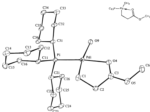
Figure 4. ORTEP diagram for [(H 2 O)Pd(CH 2 CH 2 C(O)OCH)(PCy 3 )] + [BAR' 4 ] - ( 18 ).
