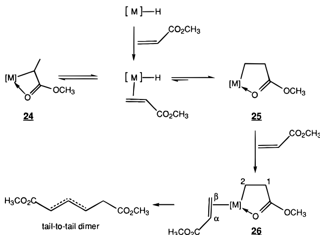
Scheme 9. A General Scheme for Selective Tail-to-Tail Acrylate Dimerization
