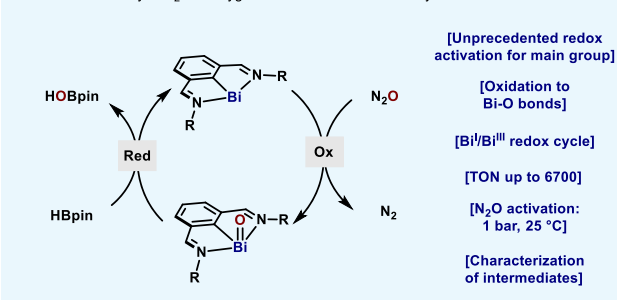
Figure 1. (A) Homogeneous N 2 O activation at centers of elements: red (stoichiometric), blue (catalytic). (B) Catalytic N 2 O deoxygenation at a Bi(I)⇌Bi(III) redox platform.
