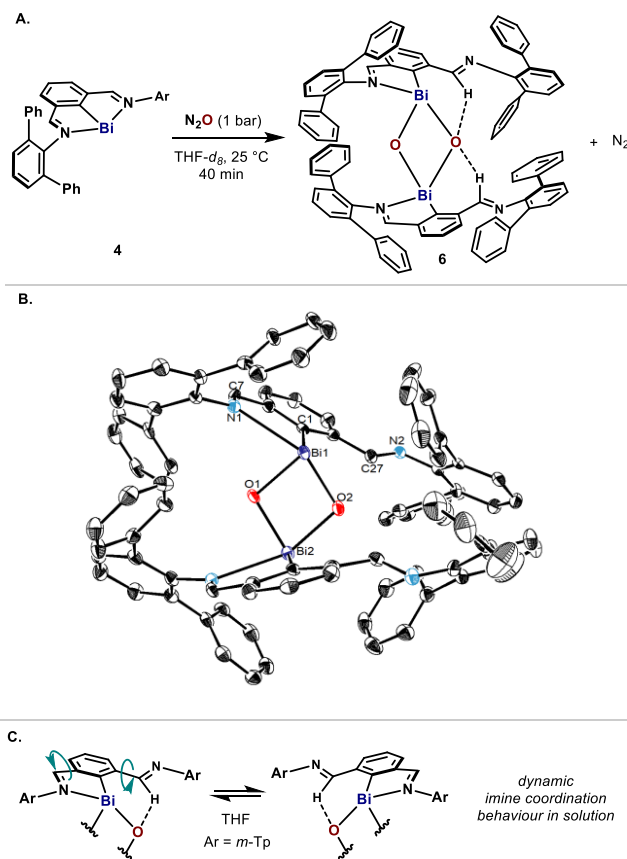
Figure 3. (A) Oxidation of bismuthinidene 4 with \text{N}_2\text{O} . (B) ORTEP drawing of 6, with ellipsoids drawn at the 50% probability level. H atoms, the toluene molecules and the enantiomer of 6 in the unit cell are omitted for clarity. Selected bond lengths (Å) and angles (deg): Bi1–C1 2.300(5), Bi1–O1 2.103(3), Bi1–O2 2.120(3), Bi1–N1 2.672(4), O1–Bi1–O2 79.70(13). (C) Dynamic imine coordination.
