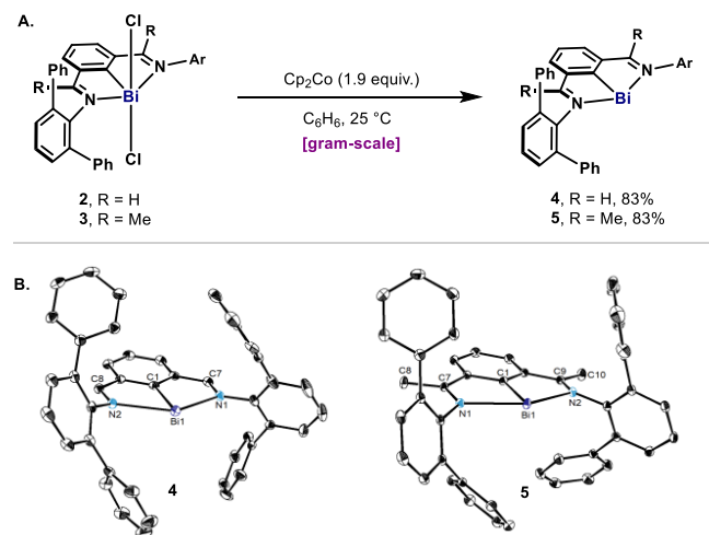
Figure 2. (A) Preparation of bismuthinidenes 4 and 5. (B) ORTEP drawing of 4 and 5, with ellipsoids drawn at the 50% probability level. H atoms of 4 and 5 as well as distortions of 4 are omitted for clarity. Ar = m -Tp. Selected bond lengths (Å): for 4, Bi1–C1 2.1487(19), Bi1–N1 2.4601(15), Bi1–N2 2.5066(15), N1–C7 1.301(3), N2–C8 1.300(2); for 5, Bi1–C1 2.1503(18), Bi1–N1 2.4621(15), Bi1–N2 2.4552(16), N1–C7 1.301(2), N2–C9 1.305(2).
