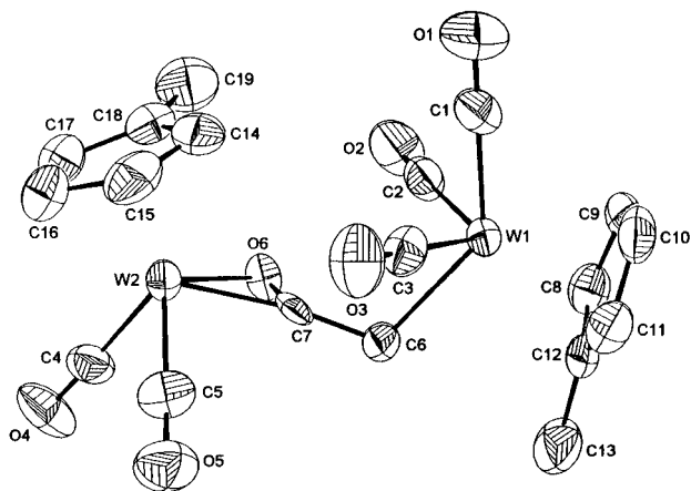
Figure 2. ORTEP drawing of (C_5H_4Me)_2(CO)_5W_2(\mu-CH_2-CO) ( 5' ) with thermal ellipsoids shown at the 50% probability level. Selected bond distances (Å) and bond angles (deg) are as follows: W(1)–C(6), 2.325(9); W(2)–O(6), 2.190(6); W(2)–C(7), 2.061(9); C(6)–C(7), 1.43(1); C(7)–O(6), 1.27(1); W(2)–C(7)–C(6), 155.6(8); C(6)–C(7)–O(6), 126.0(8); W(2)–C(7)–O(6), 78.4(5); W(2)–O(6)–C(7), 67.2(5).
