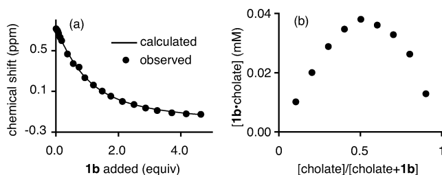
Figure 1. ^1\text{H} NMR titration (a) and Job plot (b) experiments illustrating the binding of cyclo(Adc K ) 4 to sodium cholate. In these experiments, D 2 O solutions of cyclo(Adc K ) 4 were added to a solution of sodium cholate and the chemical shift of the cholate C18 methyl group was monitored.
