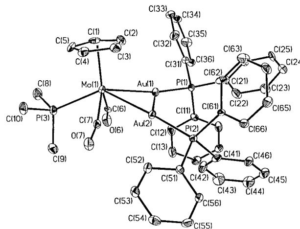
Figure 1. Top view of the [CpMo(CO) 2 (PMe 3 )(AuPPh 3 ) 2 ] + cation of compound 1 with the numbering scheme employed. Hydrogen atoms are omitted for clarity, and ellipsoids are drawn at the 40% probability level.
