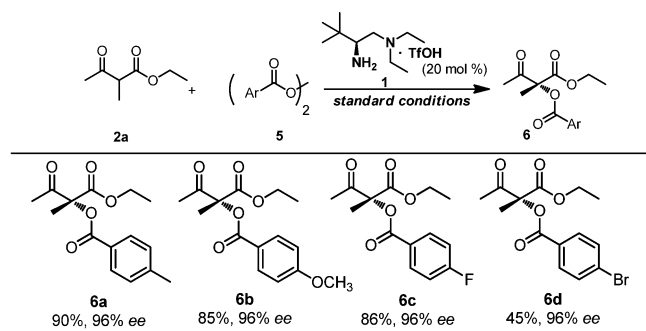
Scheme 2. Scope of Other Aryl Acylperoxides a
