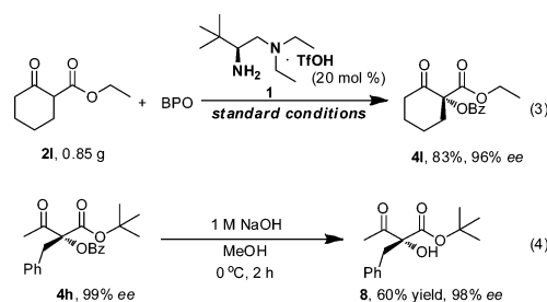
Scheme 5. Gram Scale Reaction and Synthetic Transformations
