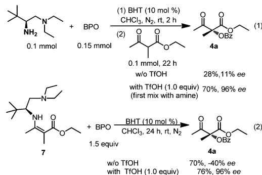
Scheme 4. Stoichiometric Experiments
