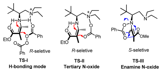
Scheme 3. Proposed Transition States
