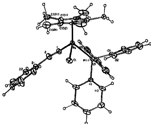
Fig. 1. Plot of a molecule of RuCl(C=CHPh)(PPh 3 )Cp * (1) showing atom numbering scheme. Selected bond parameters: Ru–Cl 2.39(1), Ru–P(1) 2.305(3), Ru–C(1) 1.80(1), Ru–C(6) (centroid of Cp * ring) 1.930(6), C(1)–C(2) 1.40(2) Å; C(1)–Ru–Cl 128.2(4), Cl–Ru–P(1) 89.2(1), P(1)–Ru–C(1) 88.5(4), Ru–C(1)–C(2) 176(1)°.
