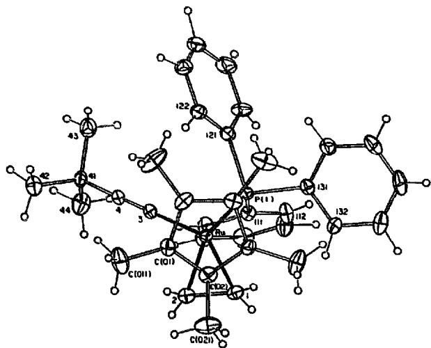
Fig. 2. Plot of a molecule of \text{Ru}(\text{C}\equiv\text{CBu}')(\eta\text{-C}_5\text{H}_4)(\text{PPh}_3)\text{Cp}^* (2) showing atom numbering scheme. Selected bond parameters: Ru–P(1) 2.300(3), Ru–C(1) 2.186(7), Ru–C(2) 2.169(7), Ru–C(3) 2.033(6), Ru–C(0) (centroid of \text{Cp}^* ring) 1.90 2 , C(1)–C(2) 1.386(9), C(3)–C(4) 1.190(8) Å; C(3)–Ru–P(1) 83.3(2), C(1,2)–Ru–P(1) 93.8(2), C(1,2)–Ru–C(3) 95.6(2), Ru–C(3)–C(4) 179.0(5), C(3)–C(4)–C(41) 174.2(7)°.
