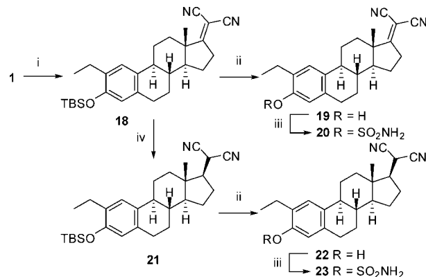
Scheme 2. Synthesis of 17-(1,1-Dicyano)methyl Estratriene Derivatives a
