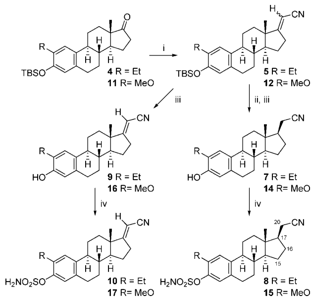
Scheme 1. Synthesis of 17-Cyanomethyl and 17-Cyanomethylene Estratriene Derivatives a
