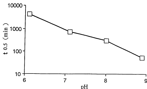
Fig. 1. Rate of Racemization of (R)-Thalidomide
