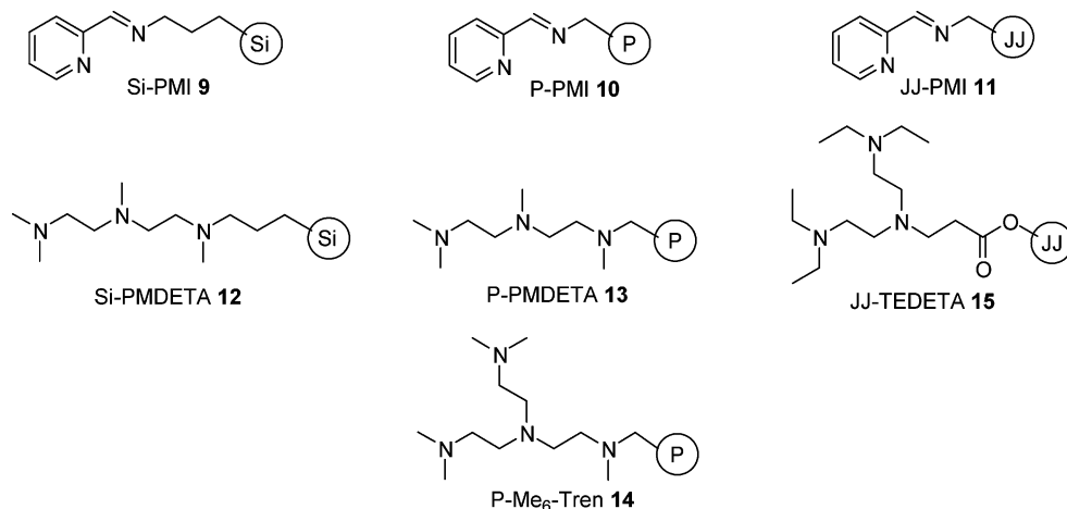
FIGURE 2. Solid-supported ligands 9–15.
