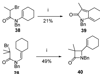
SCHEME 4. Cyclization of 28 and 38 a
