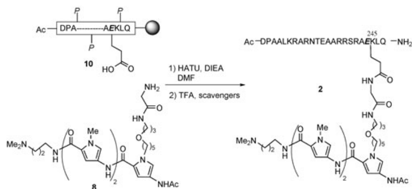
Scheme 2. Coupling step for the synthesis of 2 .
