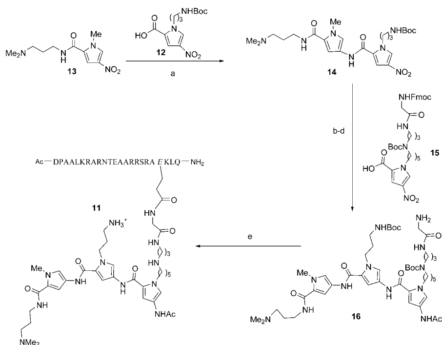
Scheme 3. Synthesis of the peptide–tripyrrole hybrid 11 . a) 1) \text{H}_2 , Pd/C; 2) DECP, \text{Et}_3\text{N} , DMAP, THF, 12 ; b) 1) \text{H}_2 , Pd/C; 2) DECP, \text{Et}_3\text{N} , DMAP, THF, 15 ; c) 1) \text{H}_2 , Pd/C; 2) \text{AcCl} , DIEA; d) piperidine/DMF; e) 1) HATU, DIEA, DMF, 10 ; 2) TFA, scavengers.
