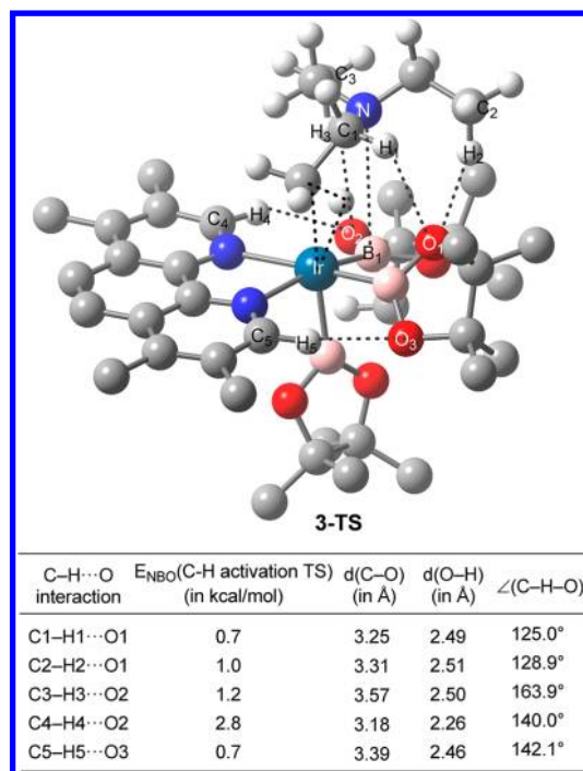
Figure 4. C–H \cdots O interactions in the transition state for C–H bond cleavage, 3-TS .
