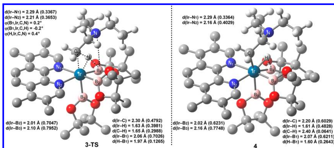
Figure 3. Structures of the transition state for C-H bond cleavage 3-TS and of the Ir-H intermediate 4. The hydrogen atoms in 3,4,7,8-Me 4 phen and Bpin ligands are deleted for clarity. The data in parentheses are the bond order for the corresponding bond.
