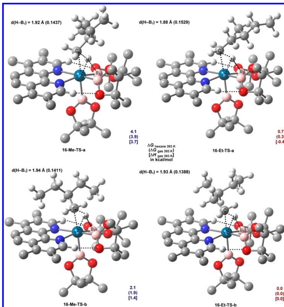
Figure 6. Transition states for cleavage of the terminal C–H bonds in 3-methylpentane.
