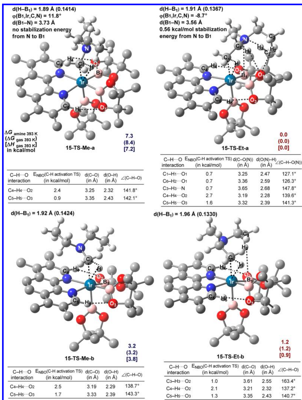
Figure 5. Transition states for C–H bond cleavage at the terminal C–H bond in methyl and ethyl groups of diethyl methylamine.
