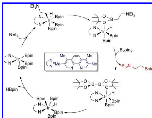
Figure 1. Proposed mechanism of the borylation of triethylamine.
