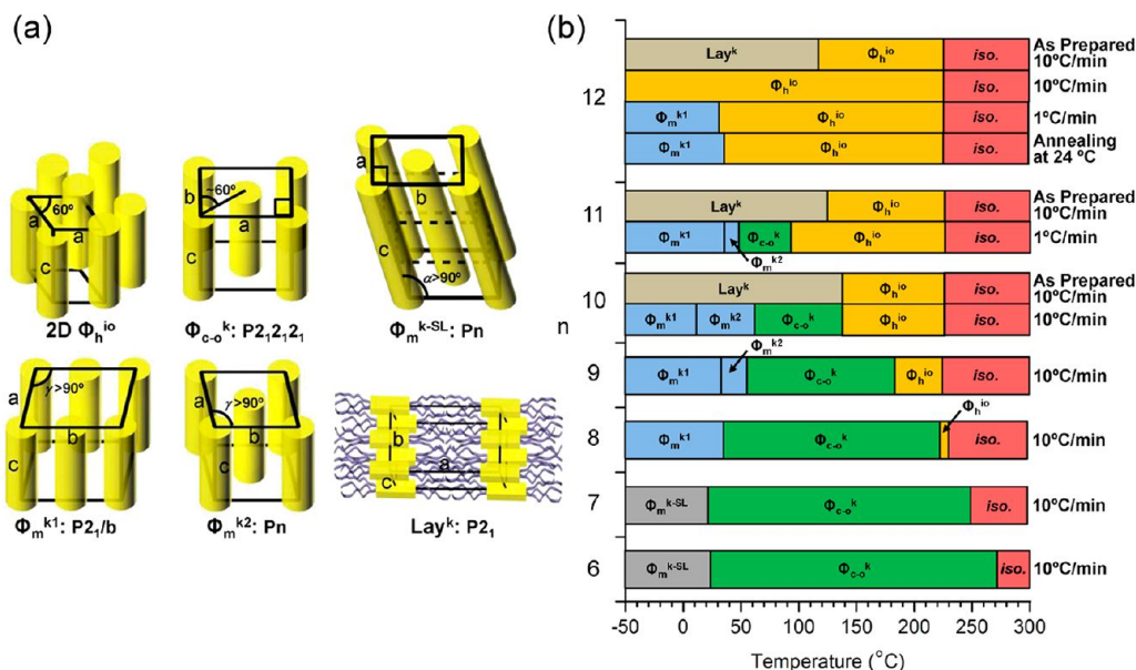
Figure 4. Schematic illustration of 2D and 3D periodic arrays self-organized from the supramolecular columns assembled from (3,4,5) n G1-1-PBI with n = 6 to 12. (a) Column arrangement of supramolecular columns in 2D and 3D lattices; their unit cell axis and angles are indicated. Phase notation: \Phi_h^{io} , 2D columnar hexagonal phase with short-range intracolumnar order; \Phi_{c-o}^k , 3D columnar center orthorhombic lattice; \Phi_m^{k-SL} , 3D columnar monoclinic crystalline superlattice; \Phi_m^{k1} , \Phi_m^{k2} , 3D columnar crystalline monoclinic phases; Lay k , layered monoclinic crystalline phase. (b) Dependence of the nature of 2D and 3D periodic arrays self-organized from (3,4,5) n G1-1-PBI as a function of n and temperature. Data were obtained from a combination of DSC and fiber and powder XRD analyses at the indicated heating rate.
