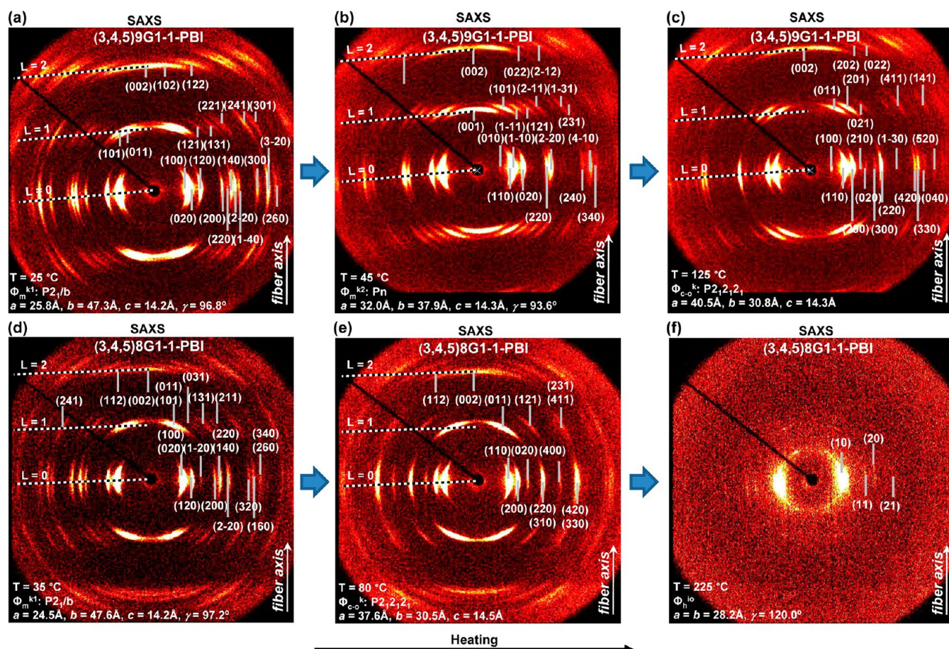
Figure 8. Small-angle XRD pattern collected from the oriented fibers of (3,4,5)9G1-1-PBI (a–c) and (3,4,5)8G1-1-PBI (d–f) during second heating with a rate of 10\text{ }^{\circ}\text{C}/\text{min} , showing the observed 3D crystalline and 2D \Phi_{h^{10}} phases at indicated temperatures. Fiber axis, symmetry, indexing, and lattice parameters of the corresponding phases are indicated.
