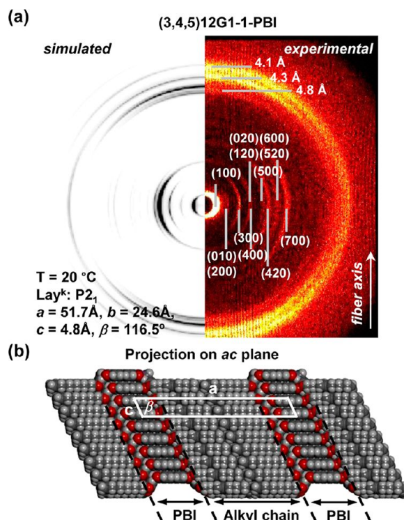
Figure 13. (a) Comparison of the experimental and simulated wide-angle XRD patterns collected from the oriented fiber of (3,4,5)12G1-1-PBI in the as-prepared condition, showing layered crystalline phase at 20 °C. Fiber axis, diffraction peaks, indexing, and lattice parameters are indicated. (b) Molecular model used in the simulation showing the construction of lamellar crystal and the layers of alkyl chain and PBI core.
