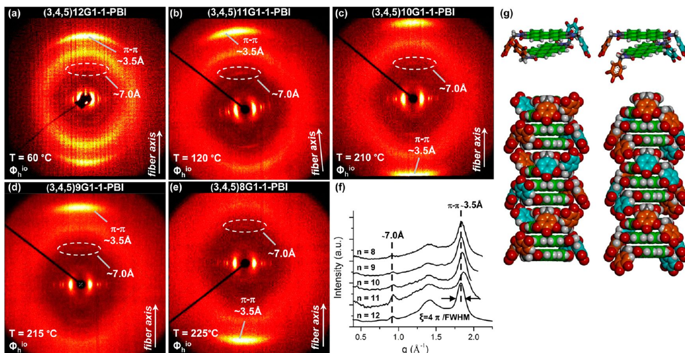
Figure 5. (a–e) Wide-angle XRD patterns collected from oriented fibers of (3,4,5) n G1-1-PBI with n = 8, 9, 10, 11, 12 in the 2D \Phi_{\text{h}}^{\text{io}} phase at the temperature shown on the diffraction patterns. Fiber axis, temperature, phase designation, and \pi – \pi stacking features are indicated. (f) The corresponding meridional plots from diffraction patterns shown in a–e. The correlation length ( \xi ) is calculated as 4\pi/\text{fwhm} , where fwhm corresponds to full width at half-maximum. (g) The two possible models of the supramolecular column. Color code: O atoms, red; H atoms, white; N atoms, blue; C atoms of the PBI, green; C atoms of the dendron phenyl, orange and light blue; all other atoms, gray.
