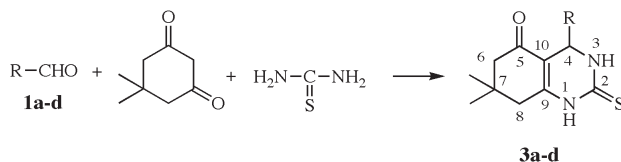
Synthesis of quinazoline derivatives
