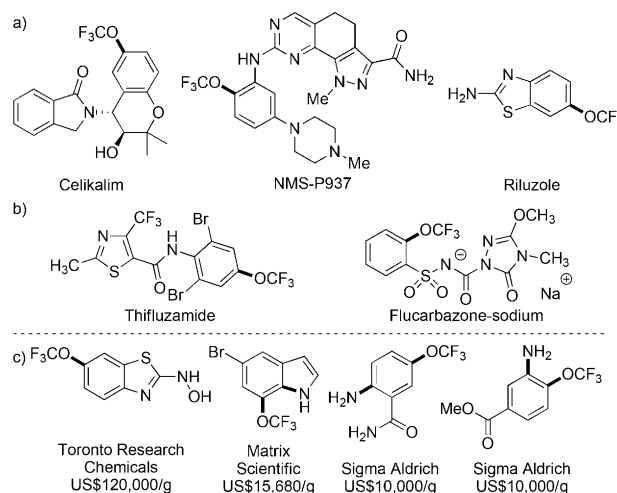
Figure 1. Examples of OCF 3 -containing a) pharmaceuticals, b) agrochemicals, and c) building blocks.
