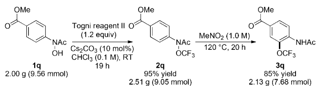
Scheme 5. Gram-scale synthesis.
