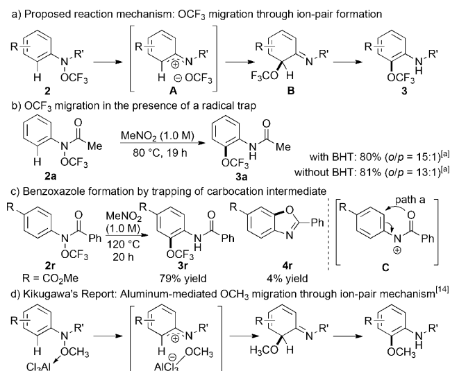
Scheme 6. Evidence for the proposed reaction mechanism. [a] 1 equiv of BHT was used. See the Supporting Information for further experimental details.
