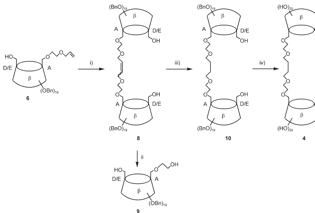
Scheme 2. Synthesis of dimer 4 . Reagents and conditions: i) [\text{Cl}_2(\text{PCy}_3)_2\text{Ru}=\text{CHPh}] (5 mol %), \text{CH}_2\text{Cl}_2 ( 10^{-1}\text{M} ), reflux, 15 h, then \text{Pb}(\text{OAc})_4 , RT, 3 h, 62 %; ii) \text{H}_2 , \text{PtO}_2 , \text{EtOAc} , RT, 3 h; iii) \text{NH}_2\text{NHTs} , \text{NaOAc} , \text{H}_2\text{O} , ethylene glycol, reflux, 6 h, 92 %; iv) Na, liq. \text{NH}_3/\text{THF} (1:1), -33^\circ\text{C} , 1 h, 96 %.
