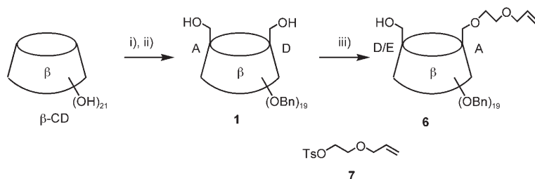
Scheme 1. Synthesis of monomer 6 . Reagents and conditions: i) BnCl, NaH, DMSO, RT, 12 h, 95 %; ii) i\text{Bu}_2\text{AlH} , toluene, 1 h, 50 °C, 84 %; iii) 7 , KH, n\text{Bu}_4\text{NI} , THF, RT, 18 h, 67 %.
