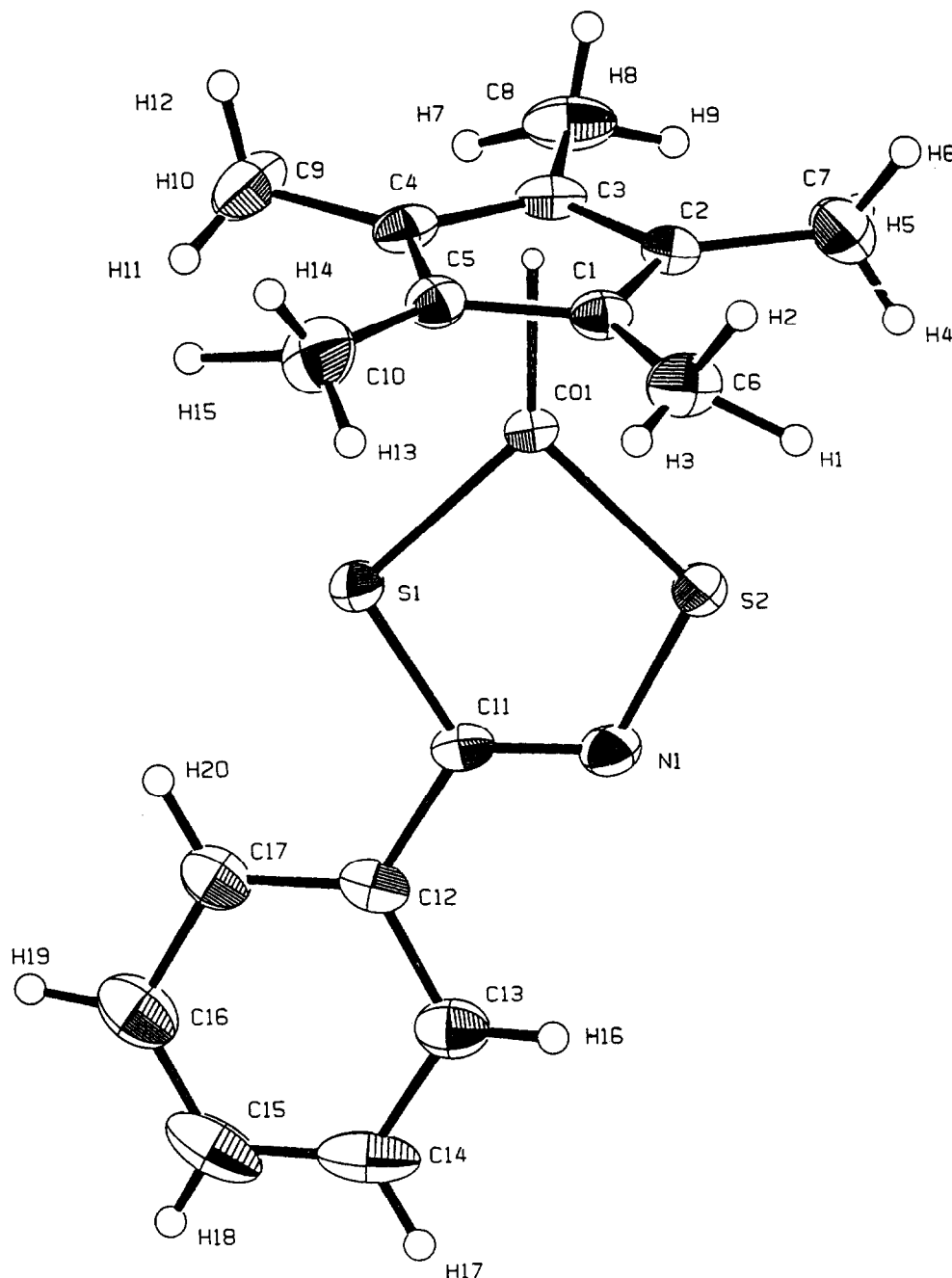
Fig. 2. Molecular structure of [(\text{cp}^*)\text{CoSN}=\text{C}(\text{Ph})\text{S}] ( 1b ) showing the atom labeling.
