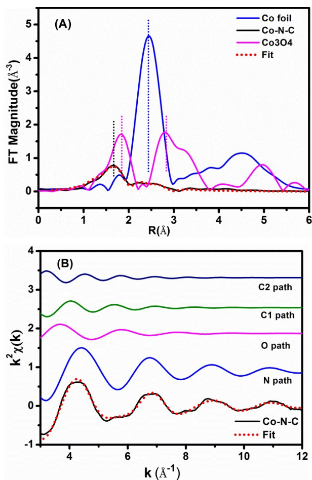
Fig. 3 (A) The k^2 -weighted Fourier transform spectra of experimental and fitting Co-N-C catalyst as well as Co foil and Co 3 O 4 reference samples. (B) The contributions of different paths including Co-N (blue line), Co-O (pink line) and Co-C (green and navy blue lines) in k-space for Co-N-C sample.
