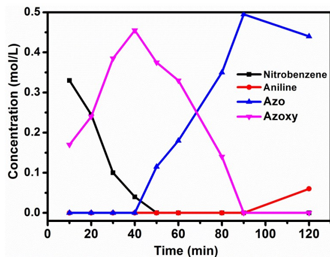
Fig. 5 Substrate and products concentration profiles as a function of the reaction time. Reaction conditions: Co-N-C catalyst: 0.7 mol%; NaOH (0.2 equiv.); solvent: t-BuOH (2 mL); 80 °C; 3 MPa H 2 .
