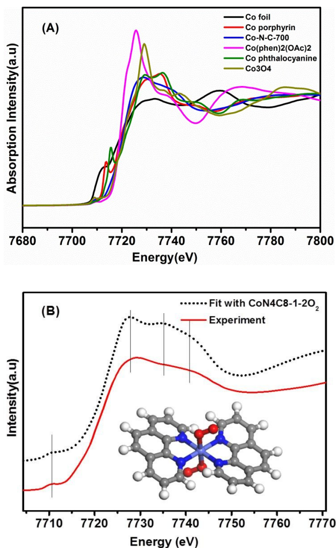
Fig. 2 (A) The normalized XANES spectra at Co K-edge of different samples. (B) Comparison between the K-edge XANES experimental spectrum of Co-N-C (solid red line) and the theoretical spectrum (black dotted line) calculated with the inset structure.
