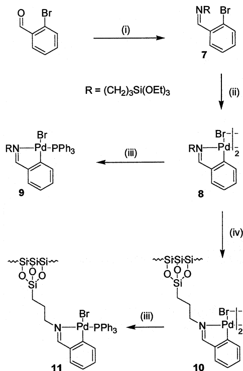
Scheme 2. (i) \text{H}_2\text{N}(\text{CH}_2)_3\text{Si}(\text{OEt})_3 , EtOH, molecular sieves; (ii) [\text{Pd}(\text{dba})_2] , toluene, 60^\circ\text{C} ; (iii) \text{PPh}_3 , \text{CH}_2\text{Cl}_2 ; (iv) silica, toluene, reflux temperature.
