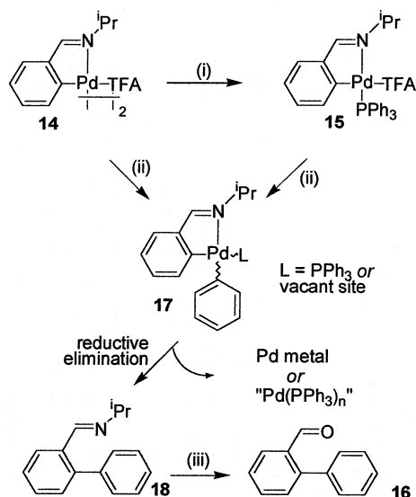
Scheme 4. (i) \text{PPh}_3 , \text{CH}_2\text{Cl}_2 ; (ii) five equivalents \text{PhB(OH)}_2 , 7.5 equivalents \text{K}_2\text{CO}_3 , toluene, reflux temperature; (iii) \text{HCl(aq)} , reflux temperature.
