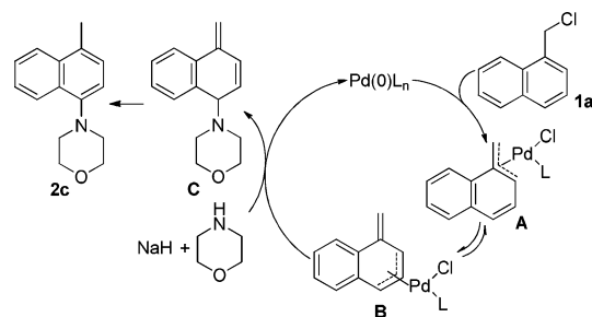
Scheme 2. Proposed Mechanism for the Palladium-Catalyzed Amination of Chloromethylnaphthalene and Chloromethylantracene Derivatives with Amines
