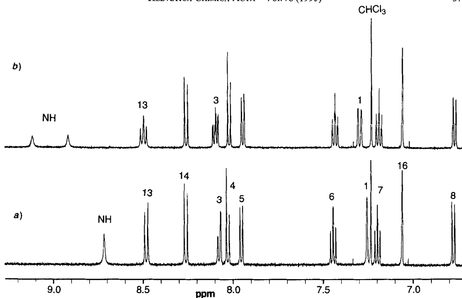
Fig. 2. Aromatic region in the 500-MHz ^1\text{H} -NMR spectra ( \text{CDCl}_3 , 300 K) of a) racemic receptor (\pm) - 3 ( c = 1.0 \text{ mM} ) and b) a mixture of (\pm) - 3 ( c = 1 \text{ mM} ) and pyranoside 22 ( c = 2 \text{ mM} )
