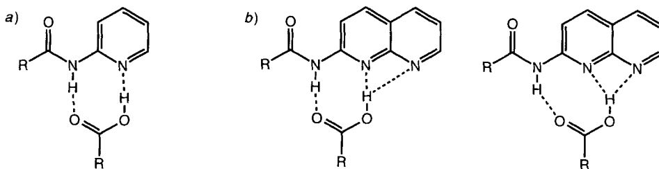
Fig. 1. Hydrogen-bonding pattern between a COOH residue and a) \text{CONH(py)} or b) \text{CONH(naphthy)} moieties
