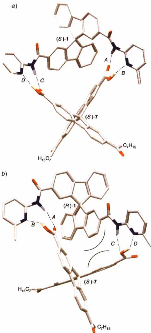
Fig. 5. Computer-generated models of the 'self-recognition' between spirobifluorene derivatives in the diastereoisomeric complexes a) (S)-1 · (S)-7 and b) (R)-1 · (S)-7, as obtained by molecular-dynamics simulations. H-Atoms are omitted for clarity.
